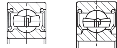
Radial contact
