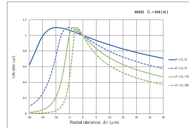
Radial clearance and bearing fatigue life
