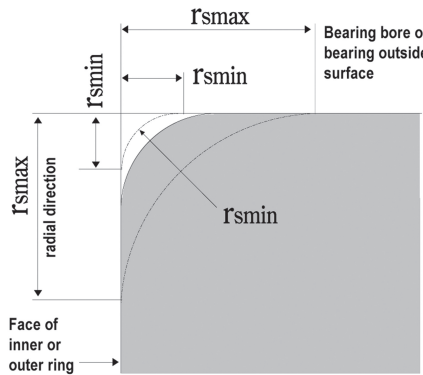
rs: Chamfer dimension of inner/outer rings
