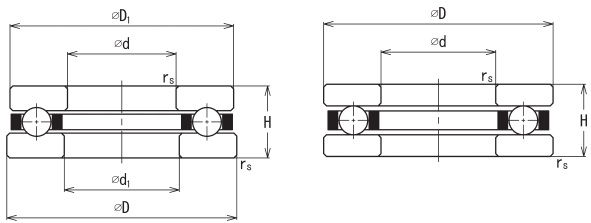
FM (with raceways) F (without raceways)
