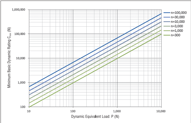
Dynamic Equivalent Load: P, Rotating Speed: n and Minimum Basic Dynamic Load Rating: C_{min}
